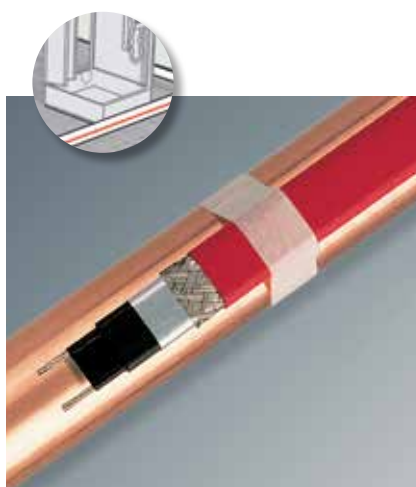
The temperature maintenance cable is attached directly on the pipe.
